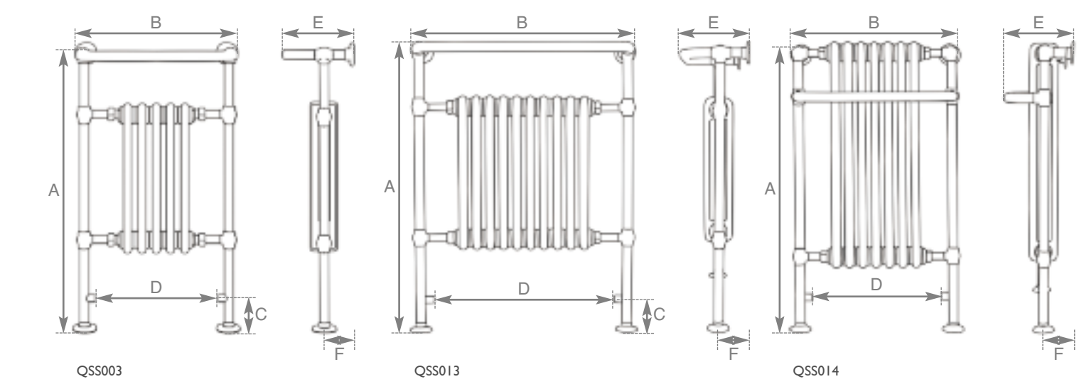
Kingston QSS014 Chrome Finish Towel Rail With White Steel Radiator
