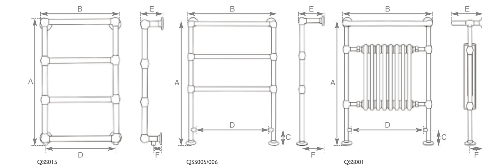
Beckingham QSS005 Chrome Finish Towel Rail Also Available: QSS006 Copper Finish Towel Rail
